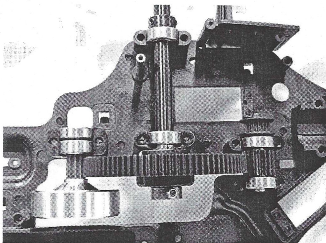
TG50_fm-brg.jpg - Caption: A peek at the main mechanics. The wider bearings are obvious.
