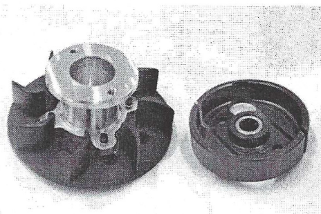
Fan and clutch assemblies. Note fan blades are more efficient airfoils, not just flat paddles. Nice attention to detail.
