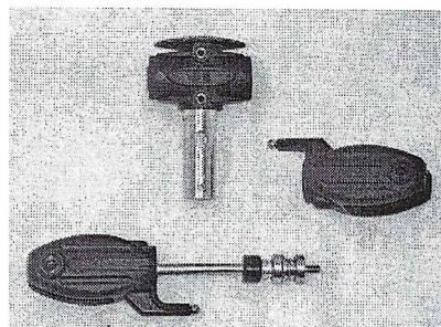
Dismantled head. Bearings are in place on shaft for photo only. Note aluminum head block.
