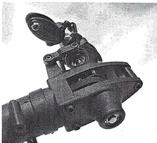
Tail rotor has an easily removable belt cage, steel hub, and a two-point tail pitch fork.
