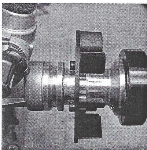
Fan/clutch assembly on engine with prop drive.
