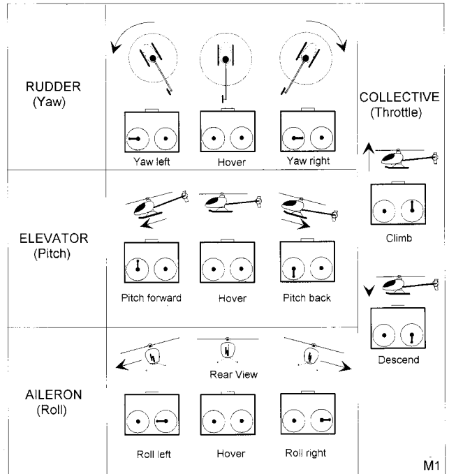
Fig. 6-3 Mode 1 Control Layout
