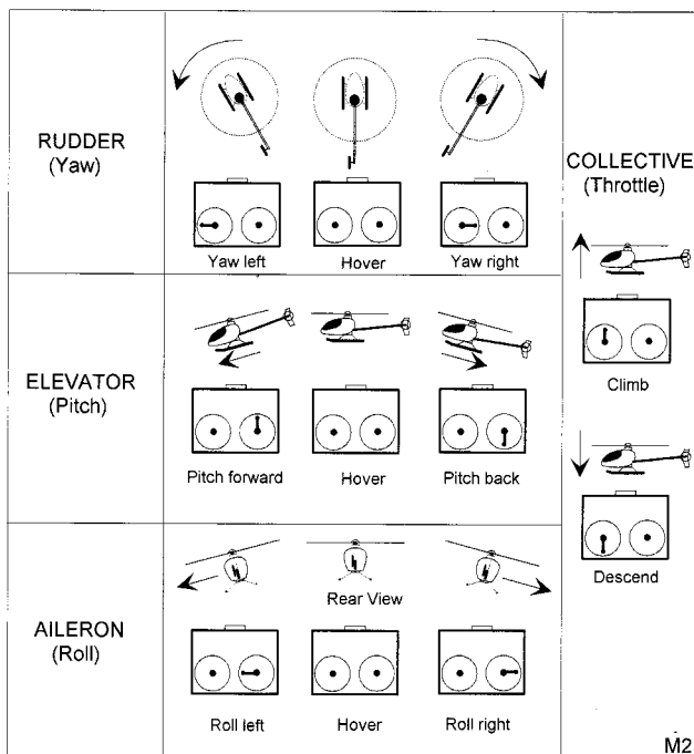
Fig. 6-2 Mode 2 Control Layout.
