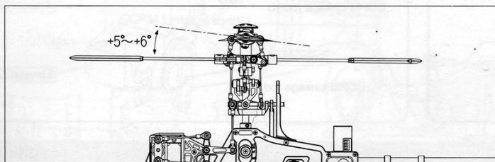
Stick position at Hovering/Throttle 65%~70%/Pitch +5^{\circ}\sim+6^{\circ}
