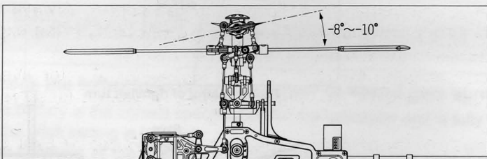
Stick position at low/Throttle 100%/Pitch -8^{\circ}\sim-10^{\circ}
