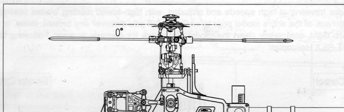
Stick position at low/Throttle 0%/Pitch 0^{\circ}
