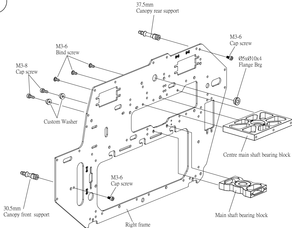
37.5mm Canopy rear support 1
