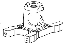
Motor mount
